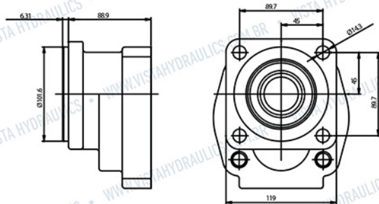
SAE B 4 Furos, ø Piloto 101.6mm (4")
